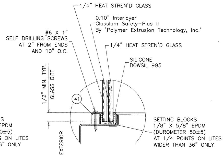
GLASS TYPE 'B1'
