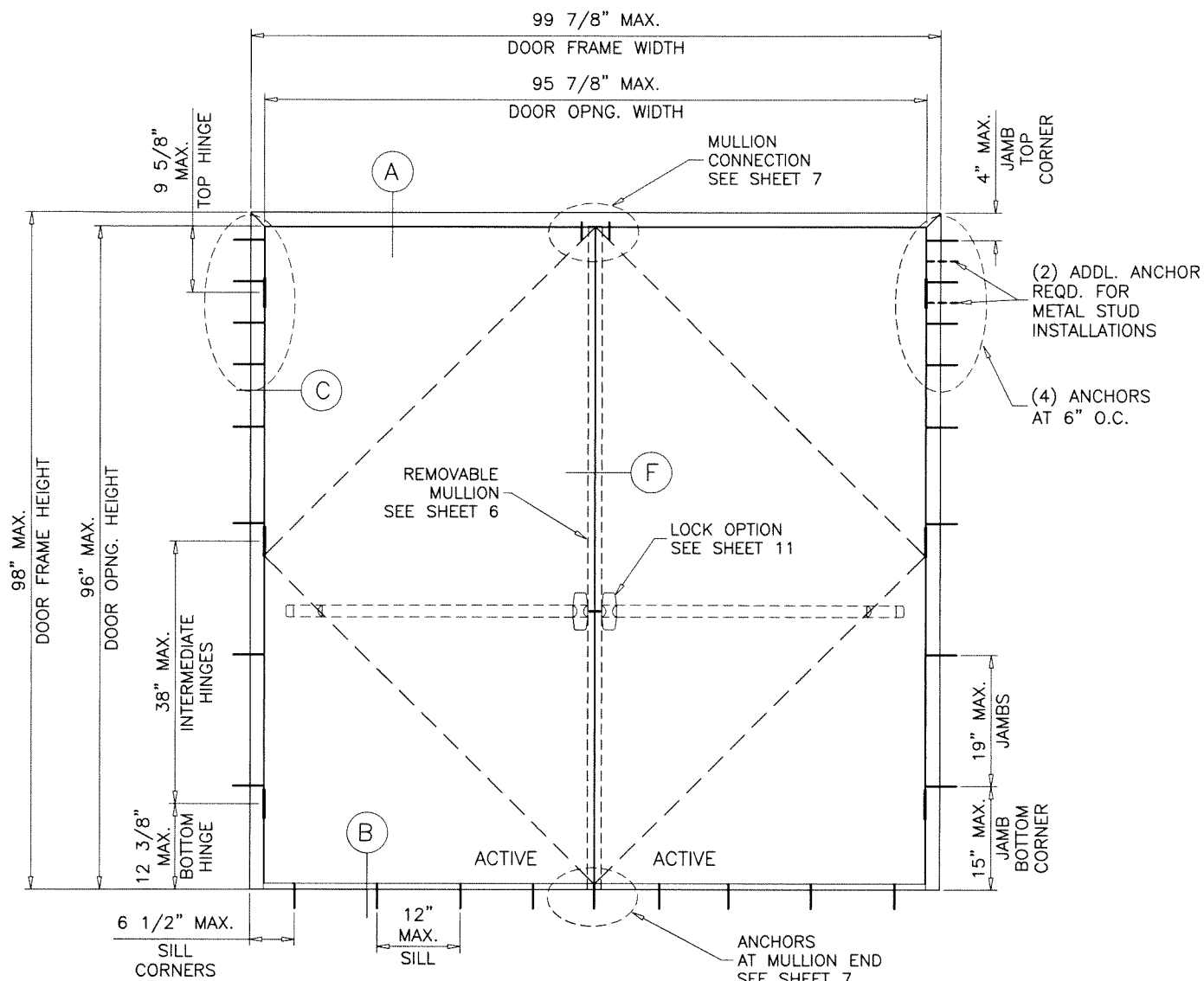
TYPICAL ELEVATION ( X-X WITH MULLION )
