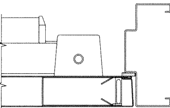
LOCK STILE SINGLE DOOR
