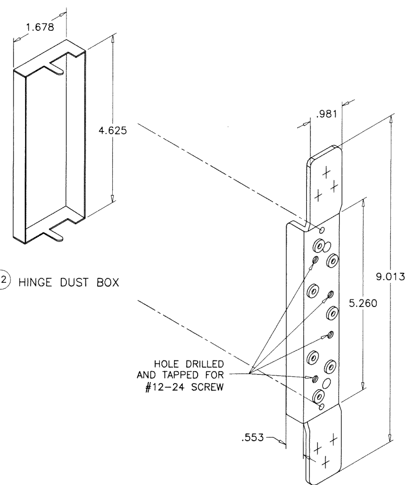
13 HINGE REINF.
