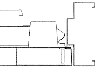
LOCK STILE SINGLE DOOR
