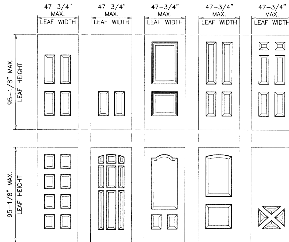
EMBOSED DOOR LEAF PATTERNS ( OPTIONAL )
