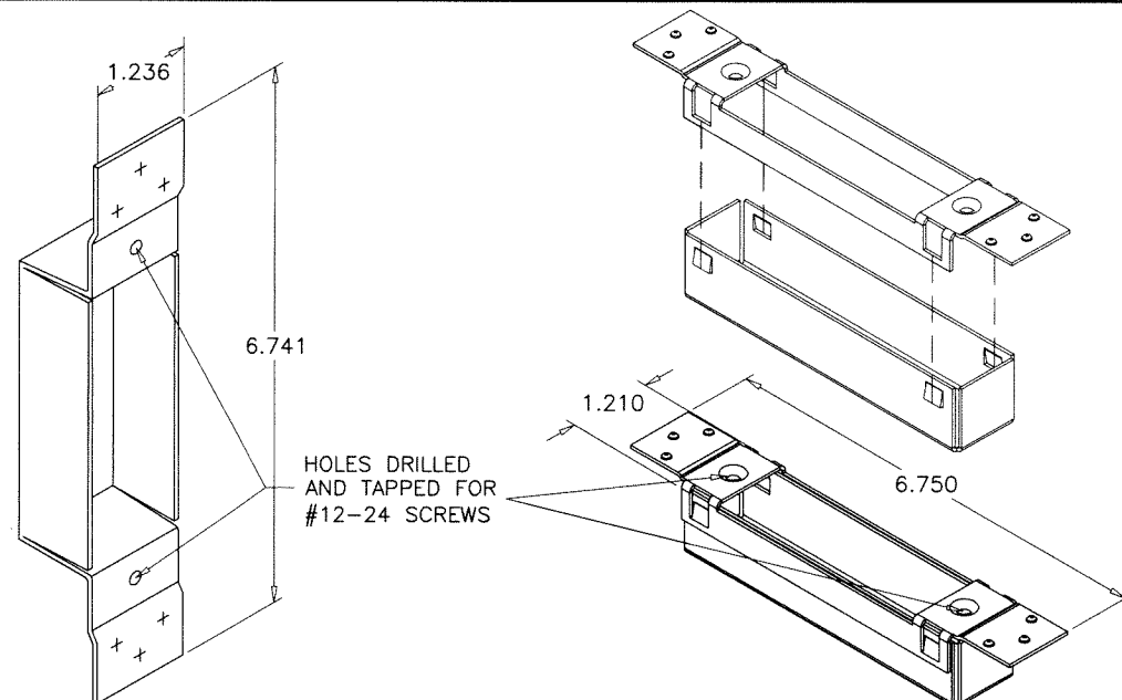
15 ASA STRIKE BOX
