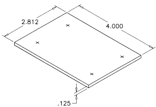
6 REINF. PLATE
