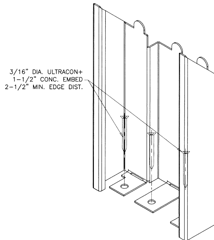
DOUBLE RABBIT FLOOR ANCHOR DETAIL OPTIONAL
