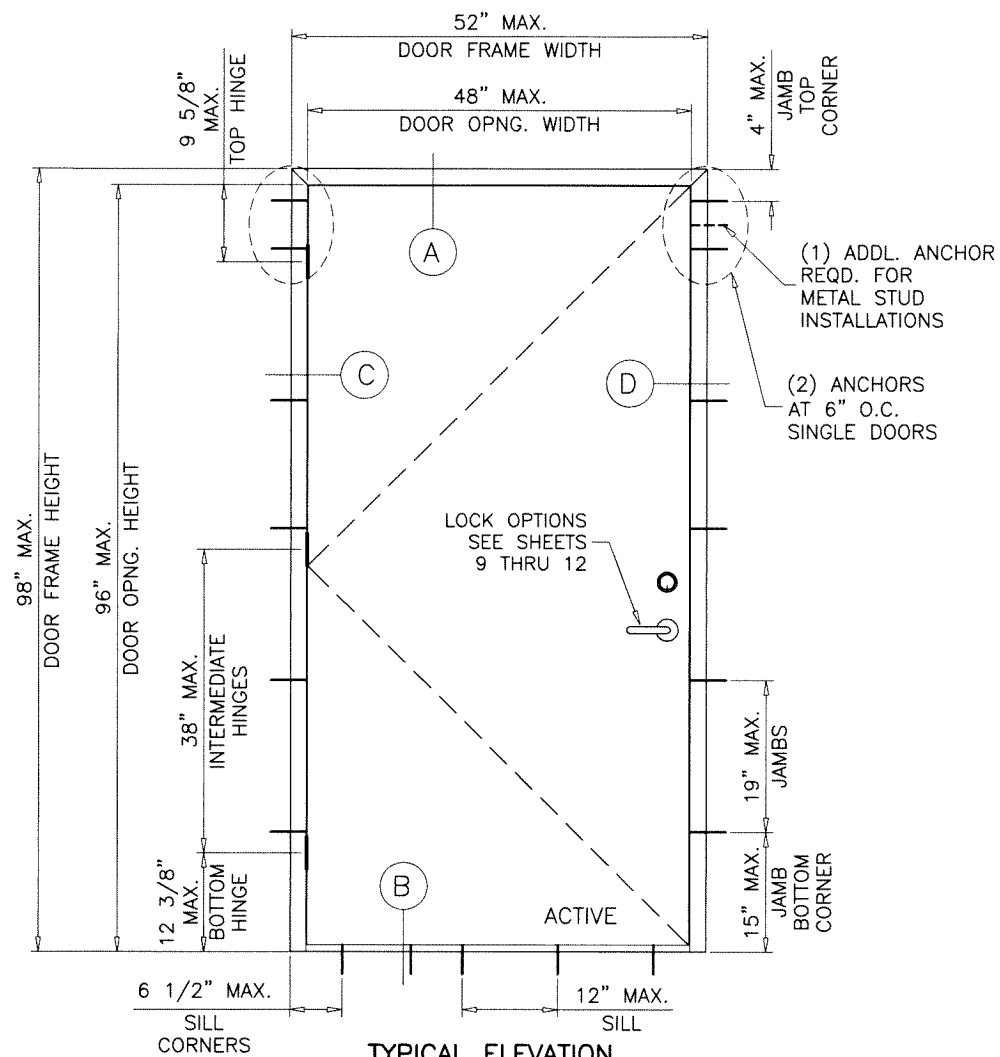
TYPICAL ELEVATION
