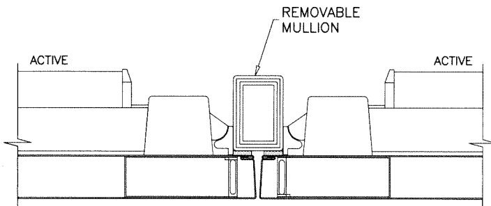
MTG. STILES DOUBLE DOOR WITH MULLION
