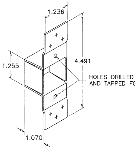
30 STRIKE REINF. DEAD BOLT
